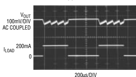
Transient Response V_{IN} = 2V , V_{OUT} = 5V
