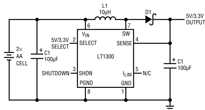
Two-Cell to 3.3V/5V Step-Up Converter
