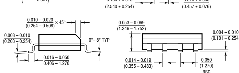
S8 Package 8-Lead Plastic SOIC
