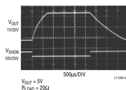
Startup Response
